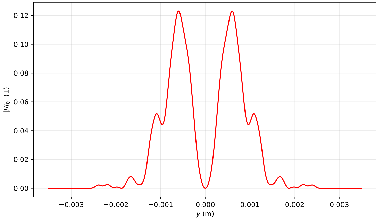
Intensity profile I(x=0, y, z=3.264)/I_0 , P_{in}=7.0P_{cr} , artificial time
